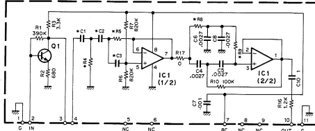
HPF (X59-4100-XX) -50 : T,T3,X,E,E9,(N)M -52 : K
