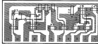
APC (X59-4090-50) Foil side view
