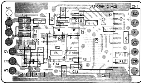
PLL (X58-398X-XX) (A/2) Foil side view
