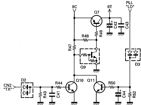
Fig. 5-2 Transmit inhibit circuit
