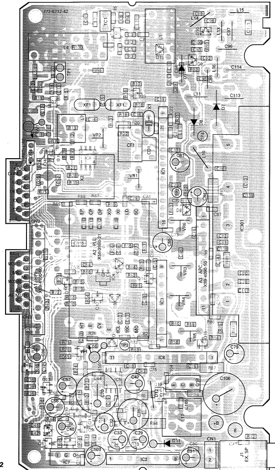
TX-RX UNIT (X57-4250-21) : TK-715(N) (M) Foil side view
