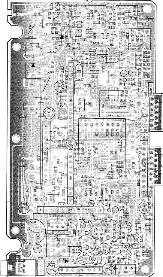
TX-RX UNIT (X57-424X-XX) Component side view
