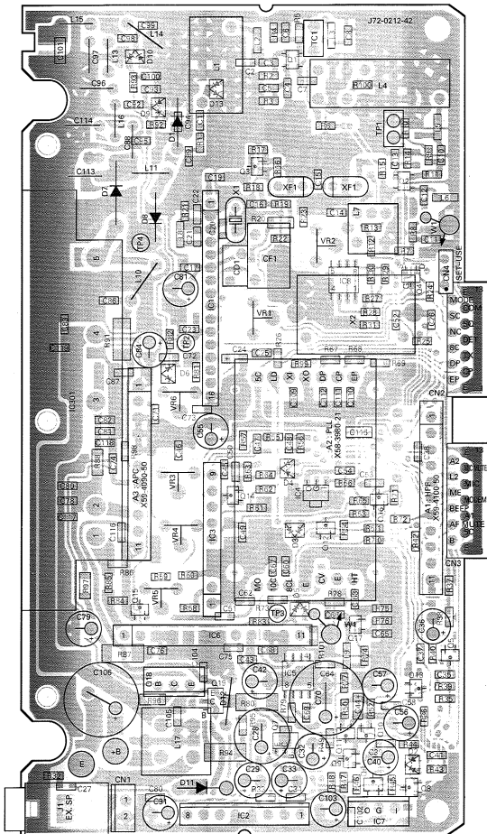
TX-RX UNIT (X57-4250-21) : TK-715(N) (M) Component side view
