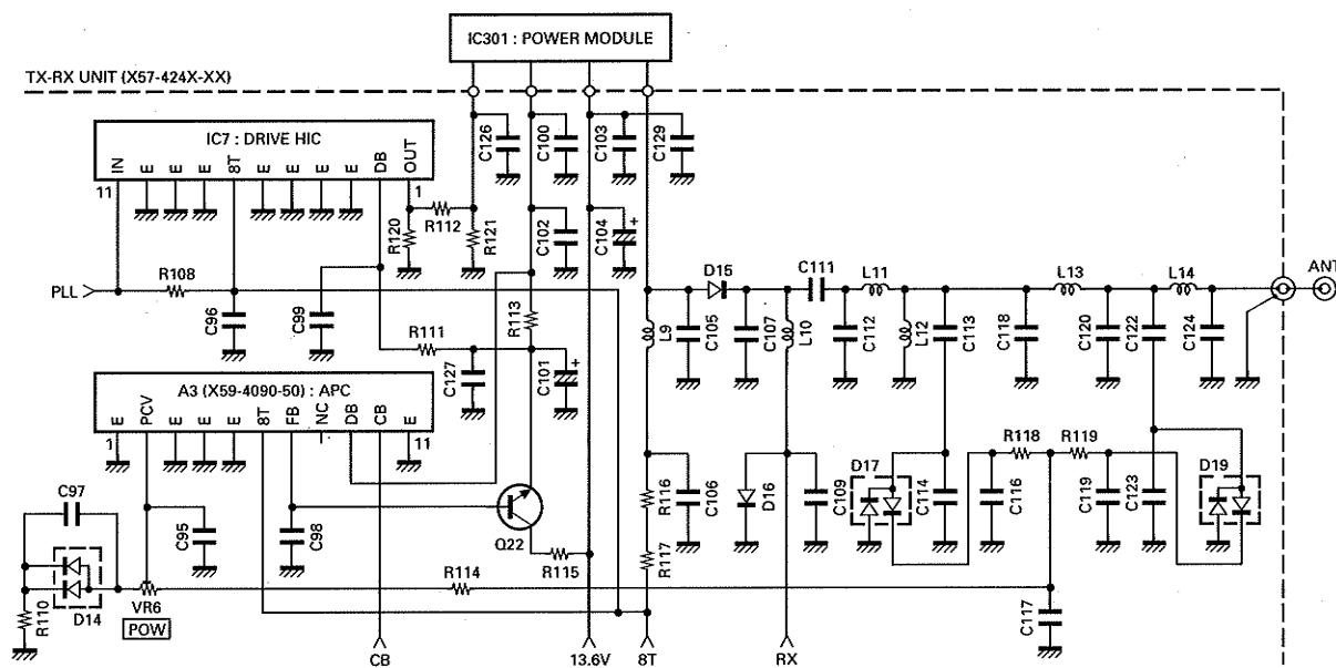
Fig. 3-1 Drive, final and APC circuits (TK-715 : K,T,T3,X,E,E9)
