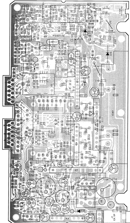
TX-RX UNIT (X57-424X-XX) Foil side view
