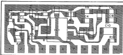
HPF (X59-4100-XX) Foil side view
